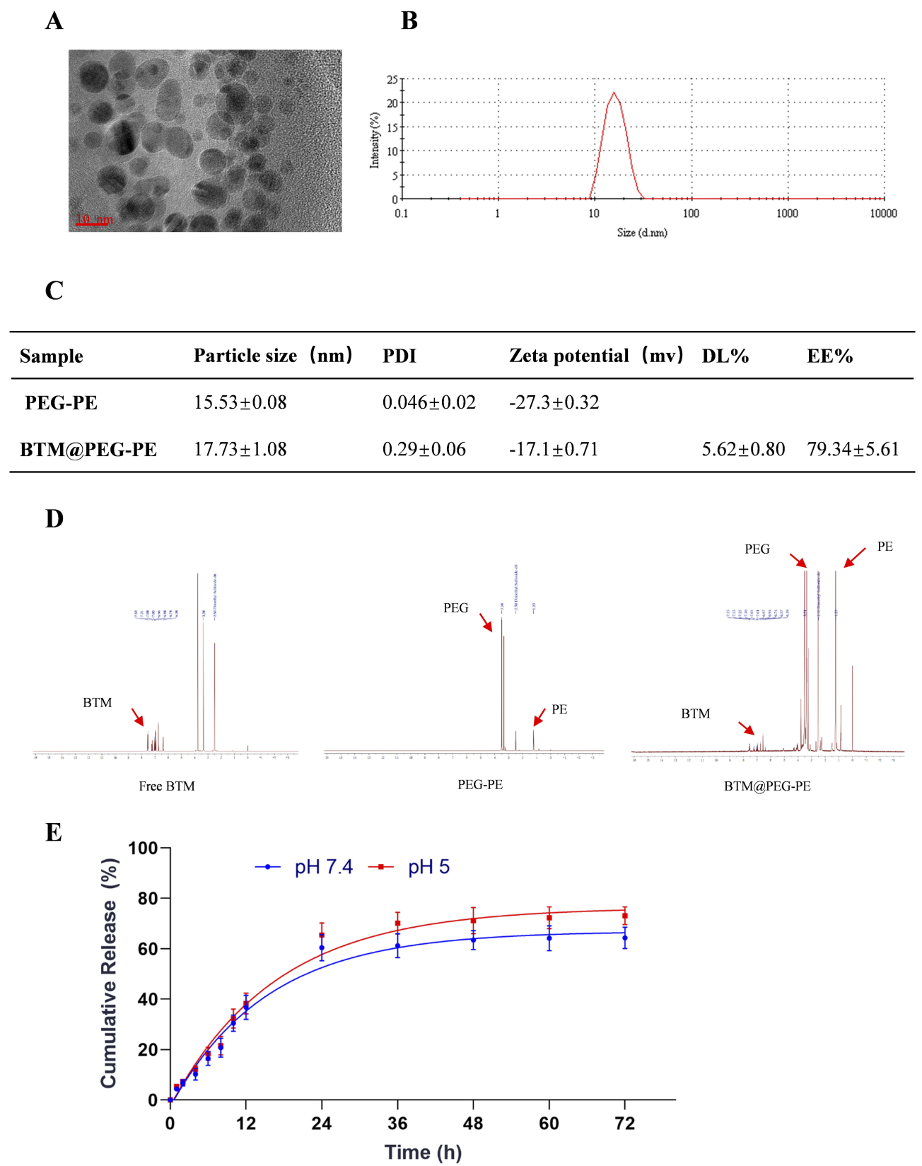
Figure 1 Characterization and loading and releasing properties of BTM@PEG-PE micelles. (A) The TEM image of BTM@PEG-PE micelles. (B) The size distribution of BTM@PEG-PE micelles. (C) Drug loading properties of BTM@PEG-PE micelles. (D) The core-shell structure of BTM@PEG-PE micelles. (E) Drug releasing properties of BTM@PEG-PE micelles at pH 7.4 and pH 5.0.
