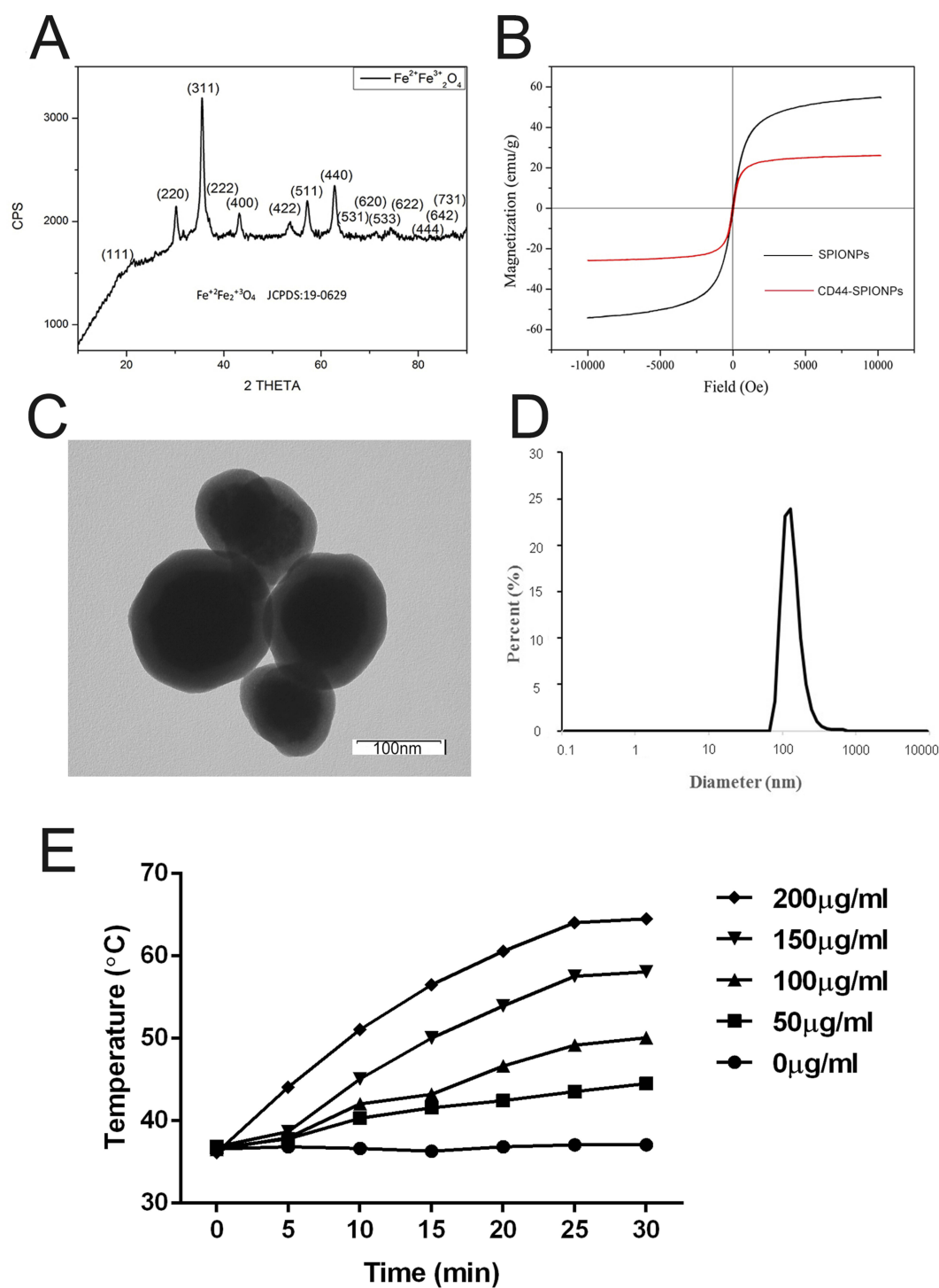
Figure 1 Characterization of SPIONs and CD44-SPIONs. (A) X-ray diffraction pattern of SPIONs. (B) Magnetization vs magnetic field curves of dry SPIONs and CD44-SPIONs at 300 K. (C) Transmission electron microscopic images of nanoparticles ( \times 80,000 ). (D) DLS analysis reporting a narrow size distribution centered at 150 nm. (E) The initial temperature was equilibrated to 37^{\circ}\text{C} , and the temperature of the CD44-SPIONs dispersion was measured using a fiber-optic temperature sensor following the application of the AMF.
