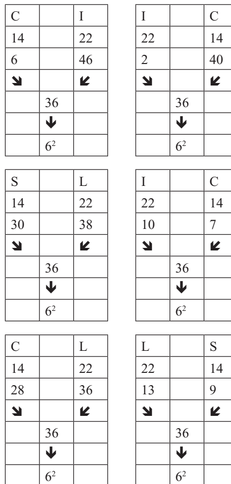
Figure 10 Distribution of amino acids according to the criteria of mathematical similarity or difference.
