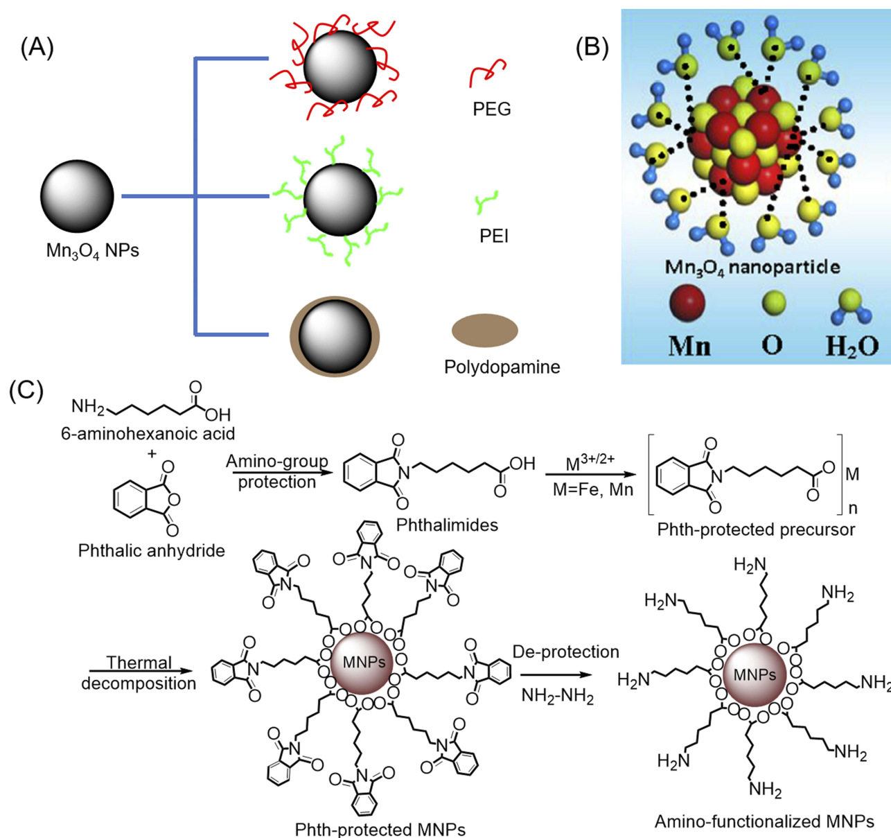
Figure 1 (A) Common modification strategy for improving the T1 relaxation rate and biocompatibility of \text{Mn}_3\text{O}_4 NPs. (B) Schematic illustration of the interaction between \text{Mn}_3\text{O}_4 NPs synthesized by liquid laser ablation and water. Reproduced from Xiao J, Tian XM, Yang C, et al. Ultrahigh relaxivity and safe probes of manganese oxide nanoparticles for in vivo imaging. Scientific Reports . 2013;3:3424. 63 (C) Synthetic route to amino-functionalized MNPs based on a protected metal-organic precursor. Reprinted with permission from Hu H, Zhang C, An L, et al. General protocol for the synthesis of functionalized magnetic nanoparticles for magnetic resonance imaging from protected metal-organic precursors. Chemistry . 2014;20(23):7160–7167. 64 Copyright © 2014 John Wiley and Sons.
