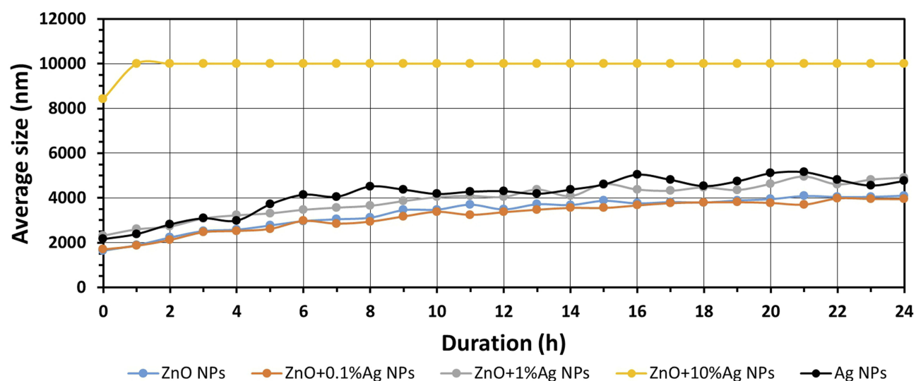
Figure 7 Results of the study of average size of NPs in artificial saliva as a function of time.
