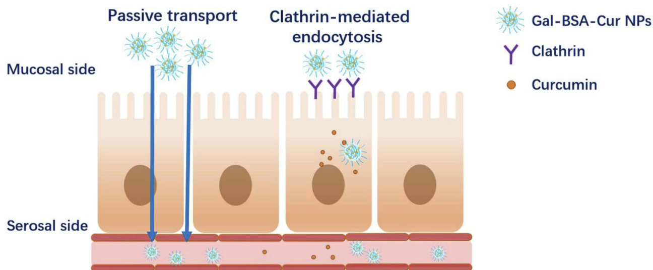
Figure 5 Scheme of the absorption mechanism used by Cur or Gal-BSA-Cur NPs.
