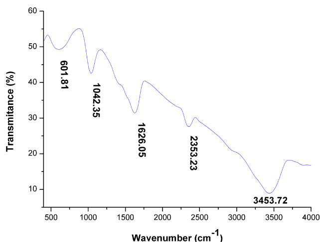
Figure 7 FTIR spectra of green SNPs synthesized using Desertifilum sp.
