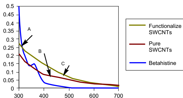
Figure 5 Ultraviolet-visible absorption spectra of A) betahistine in dimethyl-formamide (DMF), B) pure SWCNTs and, C) grafted SWCNT–betahistine (functionalized SWCNTs).
