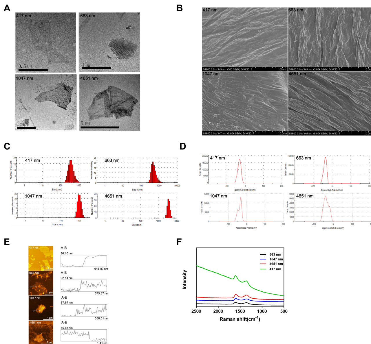
Figure 1 Characterization of graphene oxide nanoparticles. (A) TEM images of GO NPs; (B) SEM images of GO NPs. Scale Bars: 100 μm (for 417 nm)10.0 μm (for 663 nm,1047 nm and 4651 nm); (C) Size distributions of GO NPs in water; (D) Zeta potentials of GO NPs in water; (E) AFM images of GO NPs; (F) Raman spectra analysis of the GO NPs.
