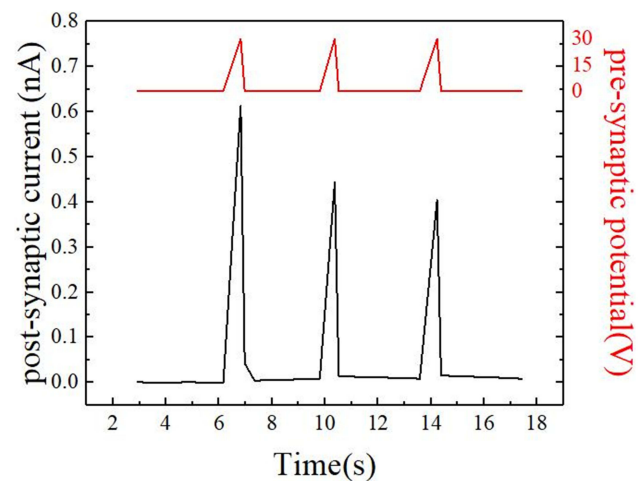
Figure 5 Experimental demonstration of paired-pulse inhibition (PPI) through the discharge current stimulated by voltage pulse on the IGZO TFT.
