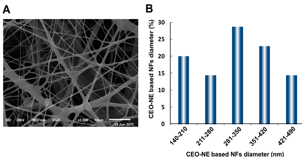
Figure 7 SEM image (A) and diameter distribution histogram (B) of CEO-NE-based NFs.
