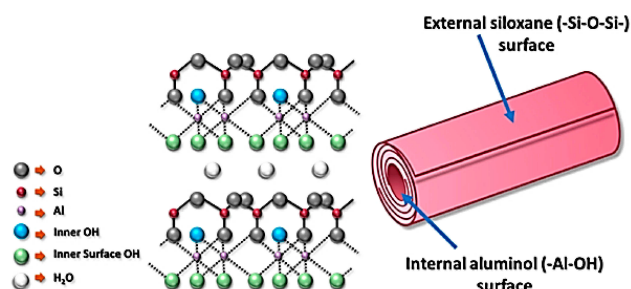
Figure 23 A schematic illustration of halloysite clay nanotubes.
