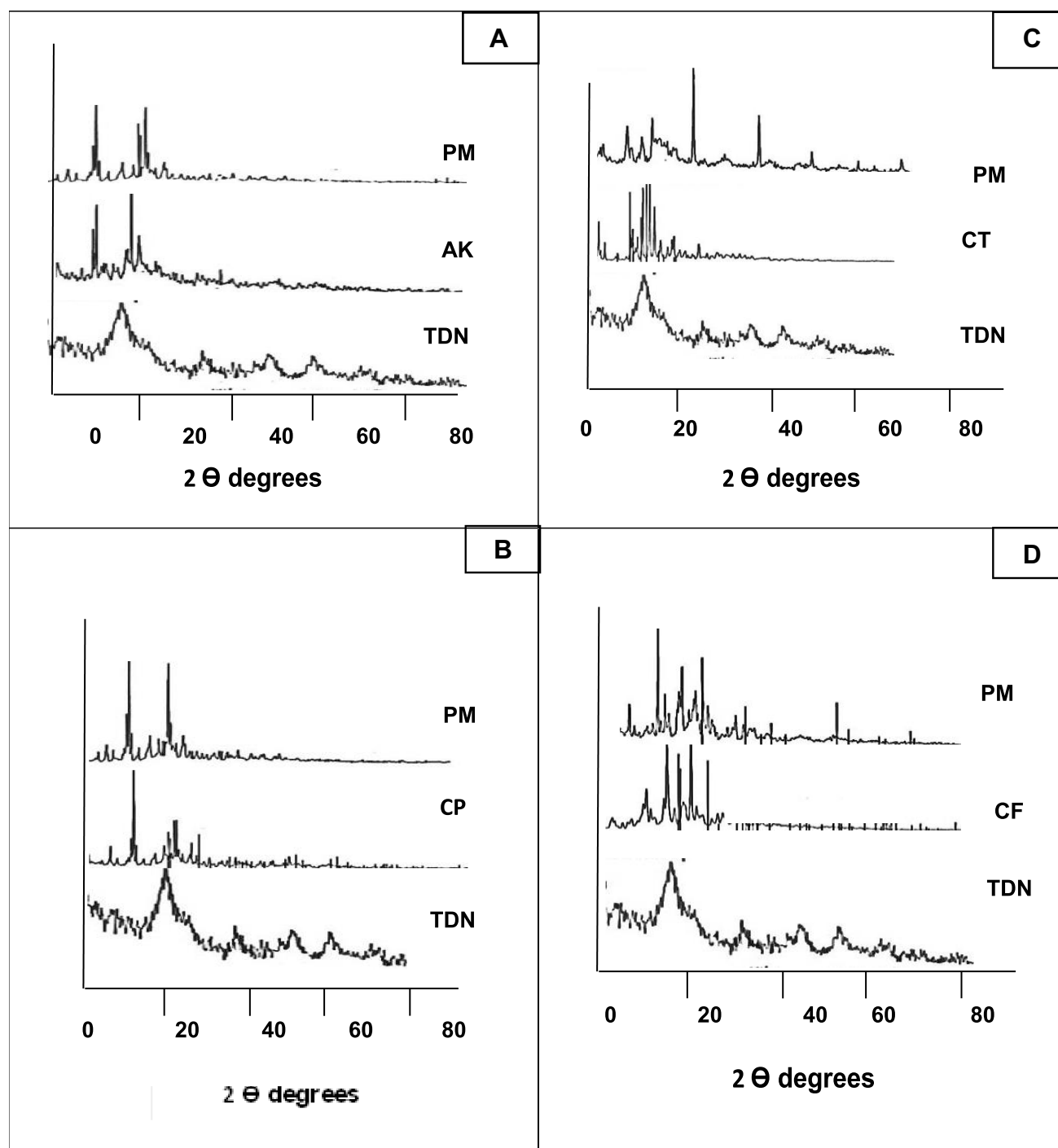
Figure 5 X-ray diffraction pattern of (A) TDN, amikacin and its physical mixture; (B) TDN, ciprofloxacin and its physical mixture; (C) TDN, ceftriaxone and its physical mixture; (D) TDN, cefpime and its physical mixture.
