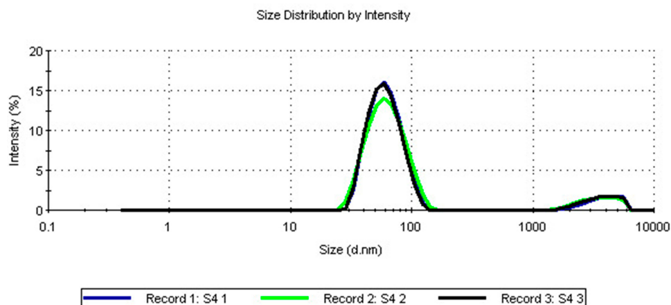
Figure 1 Particle size distribution of the formed titanium dioxide nanoparticles measured by dynamic light scattering analysis.
