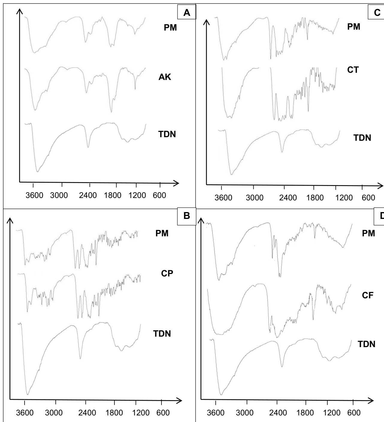
Figure 4 Fourier transform infrared spectra of (A) TDN, amikacin and its physical mixture; (B) TDN, ciprofloxacin and its physical mixture; (C) TDN, ceftriaxone and its physical mixture; (D) TDN, cefepime and its physical mixture.
