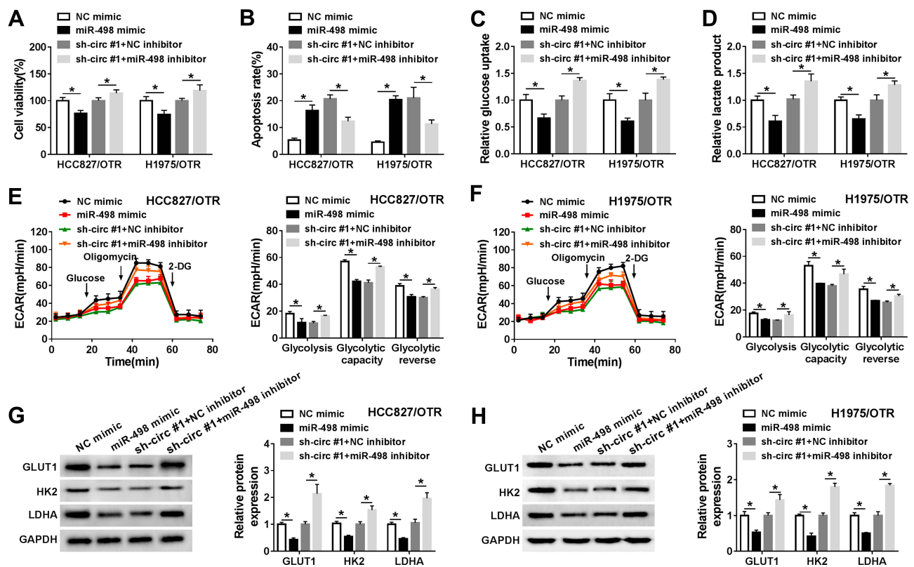
Figure 6 miR-498 deletion reversed the effects of hsa_circ_0002130 knockdown on osimertinib-resistance in osimertinib-resistant NSCLC. HCC827/OTR and H1975/OTR cells were transfected with NC mimic, miR-498 mimic, sh-circ #1+NC inhibitor or sh-circ #1+miR-498 inhibitor. (A) Cell viability was detected by MTT assay. (B) Cell apoptosis was measured by flow cytometry analysis. (C–D) The levels of glucose uptake and lactate production were determined by glucose uptake colorimetric assay kit and lactate assay kit II, respectively. (E–F) The level of ECAR was examined by Seahorse Extracellular Flux Analyzer XF96 assay. (G–H) Western blot analysis was used to detect the expression of GLUT1, HK2 and LDHA. * P < 0.05 .
