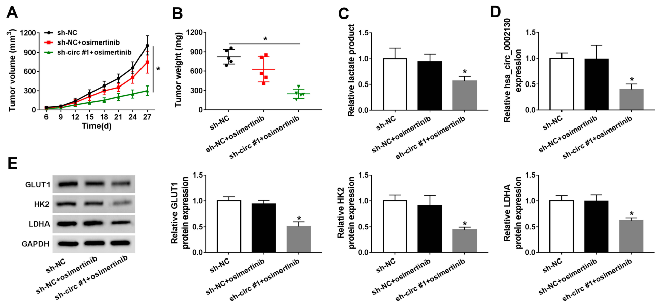
Figure 4 hsa_circ_0002130 knockdown suppressed tumor growth in vivo. (A–B) The tumor volume and tumor weight were measured. (C) The lactate production was detected by lactate assay kit II. (D) The expression of hsa_circ_0002130 was determined by qRT-PCR. (E) The expression of GLUT1, HK2 and LDHA was examined by Western blot analysis. * P < 0.05 .
