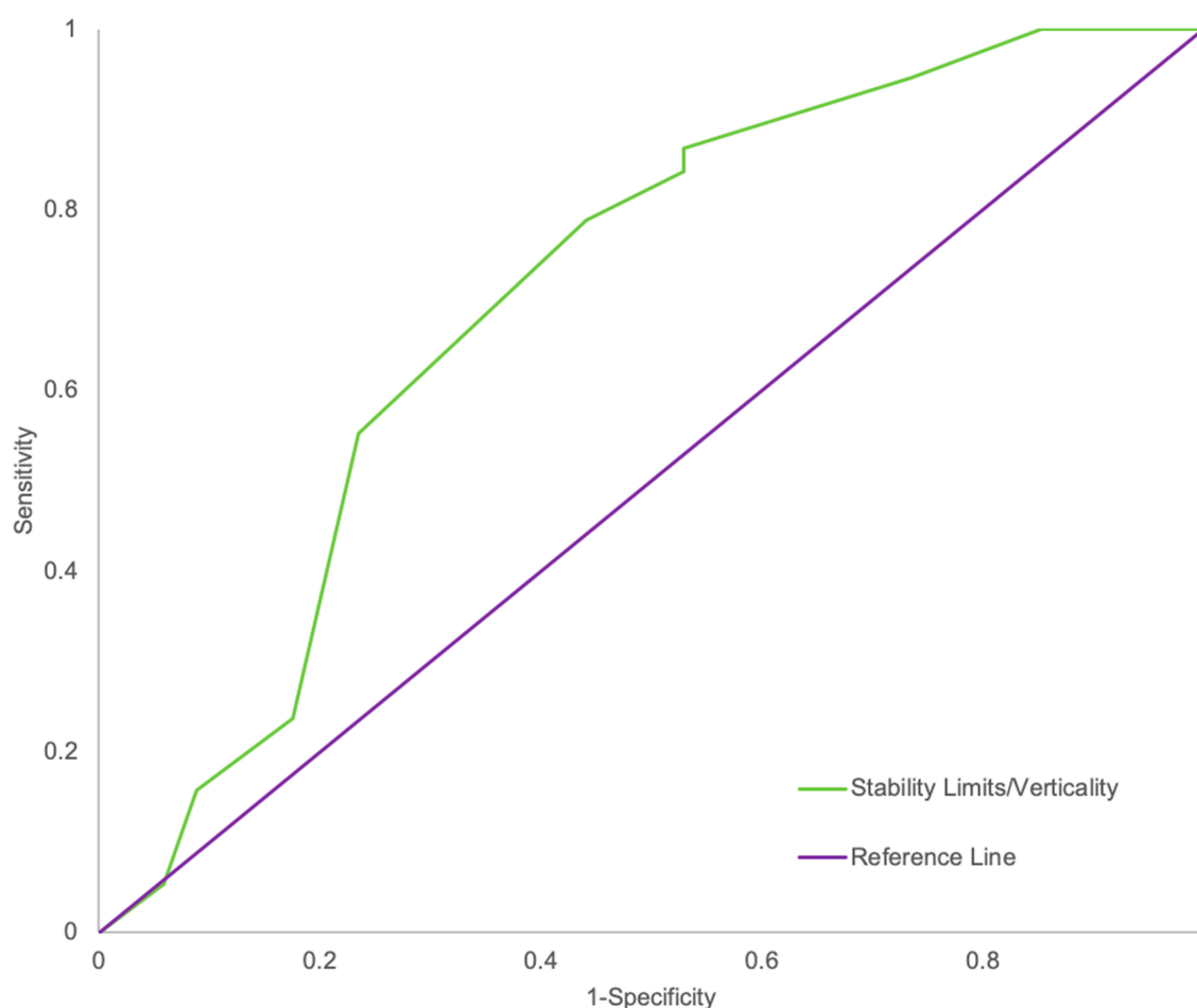
Figure 2 ROC curve for stability subcomponent score for identifying fallers with COPD.
