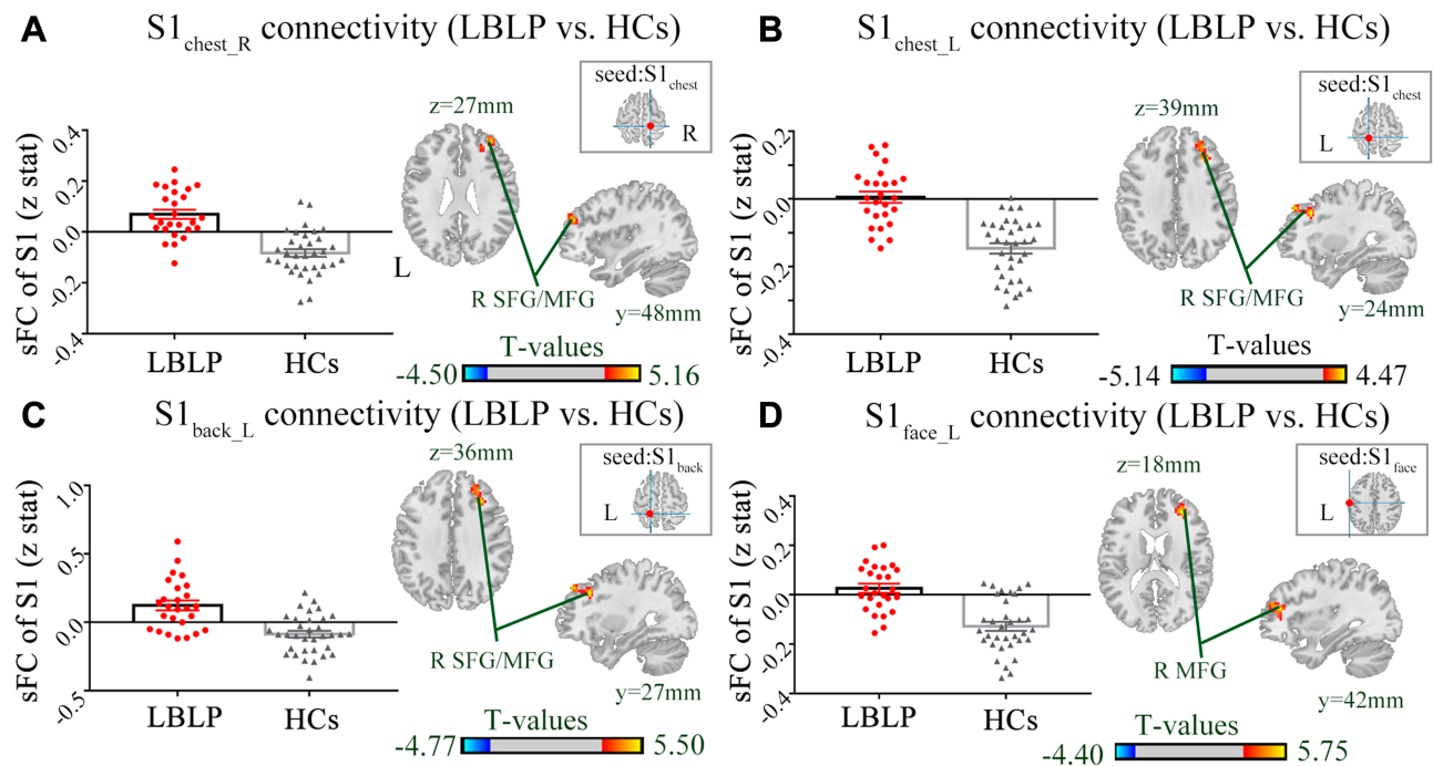
Figure 2 Differences in the alterations of sFC between the LBLP patients and healthy controls (two-sample t-test, two-tailed, voxel-level P < 0.001 , GRF correction, cluster-level P < 0.005 ).
