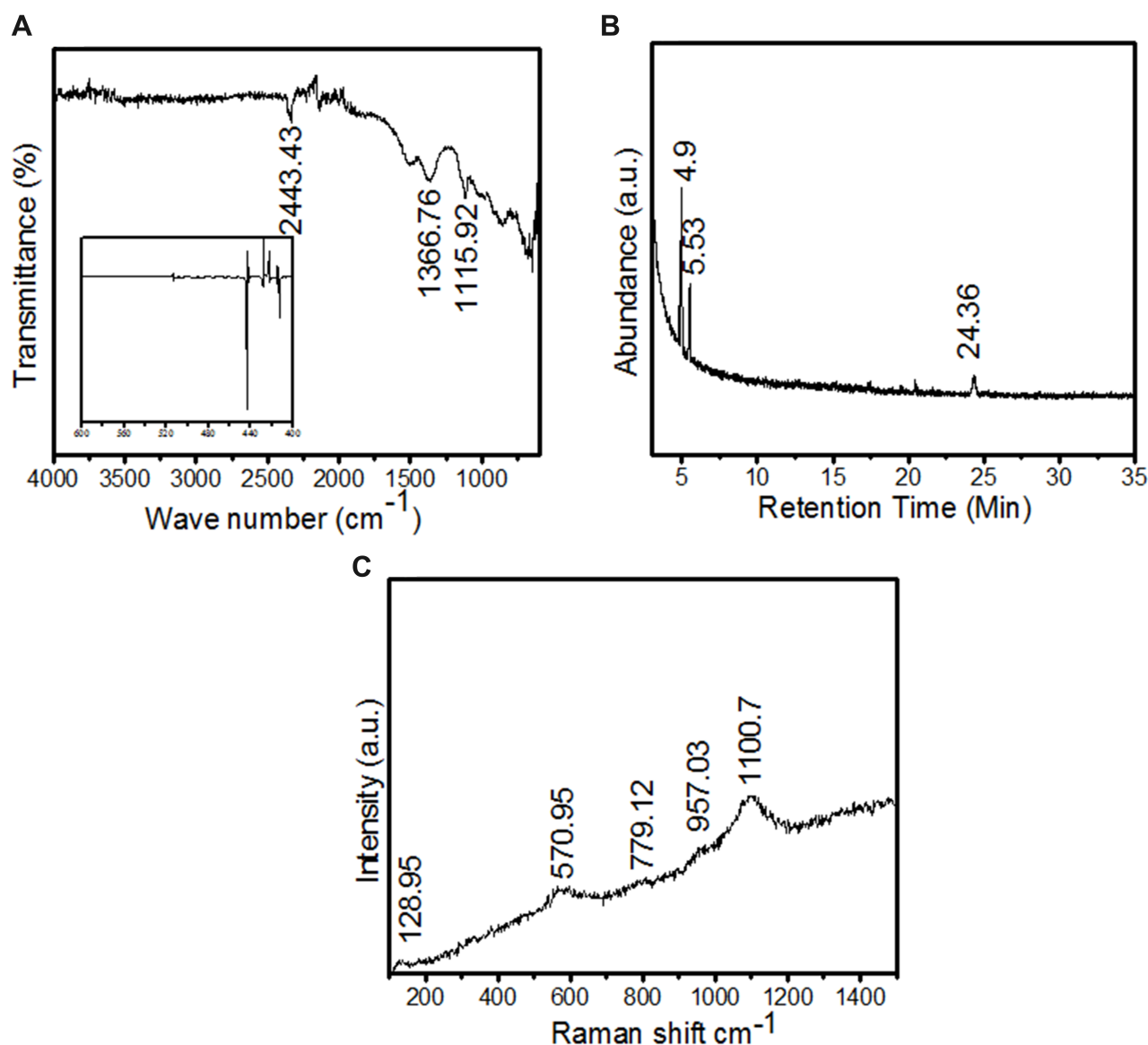
Figure 1 The demonstration of phytofunctional groups of \text{MoO}_3\text{-NiO-PdO-Pd} nanomaterial by (A) FTIR and (B) GC-MS and (C) Raman spectrum of \text{MoO}_3\text{-NiO-PdO-Pd} nanomaterial.
