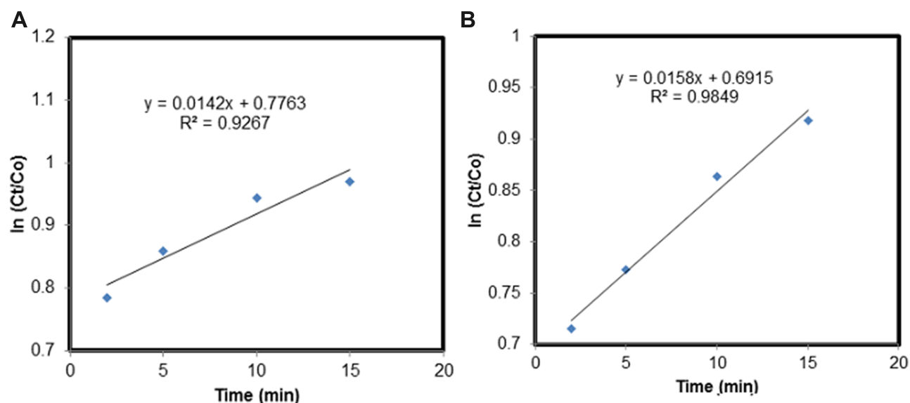
Figure 5 A plot of \ln(C_t/C_0) vs time presenting the reaction kinetic of MoO 3 -NiO-PdO-Pd (A) in presence of light, and (B) in ambient dark conditions.
