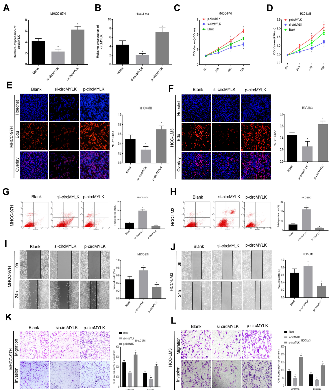
Figure 2 circMYLK promotes HCC cell migration, invasion, and proliferation while attenuating apoptosis. (A–B) qRT-PCR was carried out to detect the transfection efficiency of si-circMYLK and p-circMYLK in the MHCC-97H and HCC-LM3 cell lines. Both showed successful transfection. (C–D) The effect of si-circMYLK and p-circMYLK on the proliferation of HCC cell lines as examined by CCK-8 assays. (E–F) EdU assays for the assessment of cell proliferation ability. (G–H) Flow cytometry assessment of apoptosis levels in HCC cells. (I–J) Wound healing assay for evaluating the HCC cell migration capacity following transfection. (K–L) Transwell assays were performed to detect the migration and invasion ability of HCC cells from each group. *P < 0.05 compared with a blank group.
