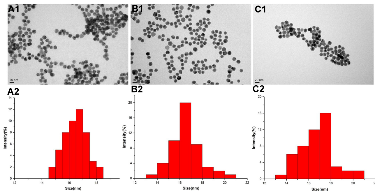
Figure 2 Transmission electron microscopic (TEM) image and size distribution of AuNPs (A1 and A2), 356-AuNPs (B1 and B2) and 356-TAT-AuNPs nm (C1 and C2).
