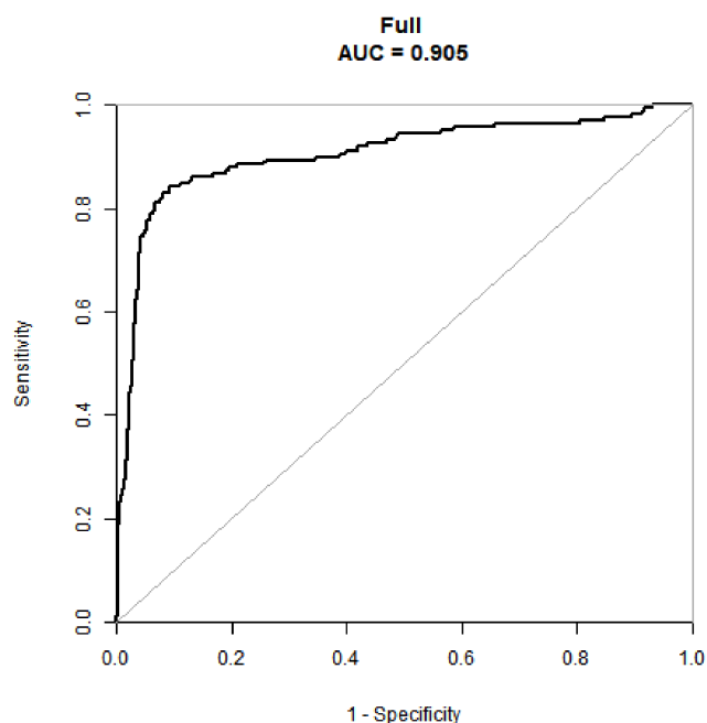
Figure 2 ROC curves for validating the discrimination of the nomogram prediction model.
