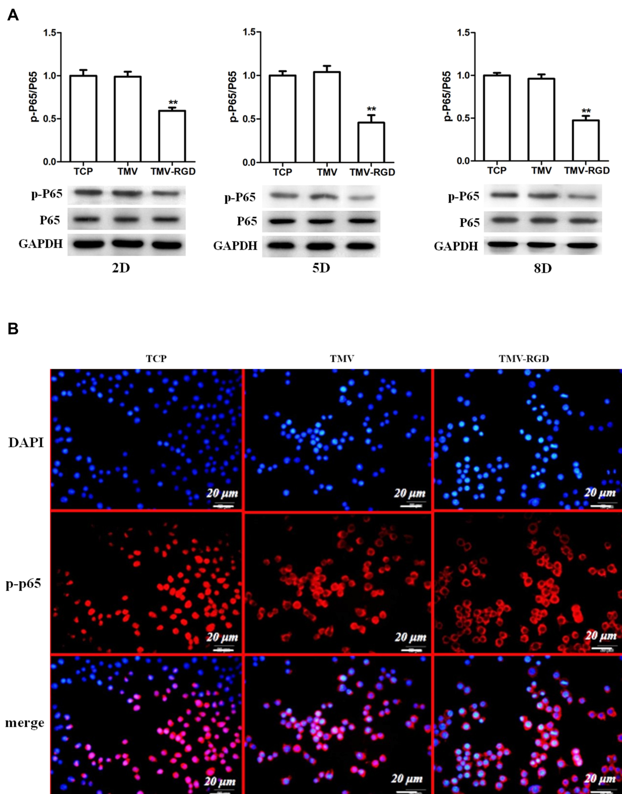
Figure 3 TMV VNPs inhibited NF- \kappa B activation. (A) Phosphorylation of NF- \kappa B p65 at different time of osteoclast differentiation was evaluated by immunoblotting. (B) The cellular localization of NF- \kappa B p65 of Raw264.7 cells was assessed by immunocytofluorescence 24 h after RANKL (50 ng/mL) treatment. NF- \kappa B p65 of cells cultured in naked plates mostly located in nuclear while that of cells in TMV and TMV-RGD coated plates mostly resided in cytoplasm. ** p < 0.01 compared to TCP.
