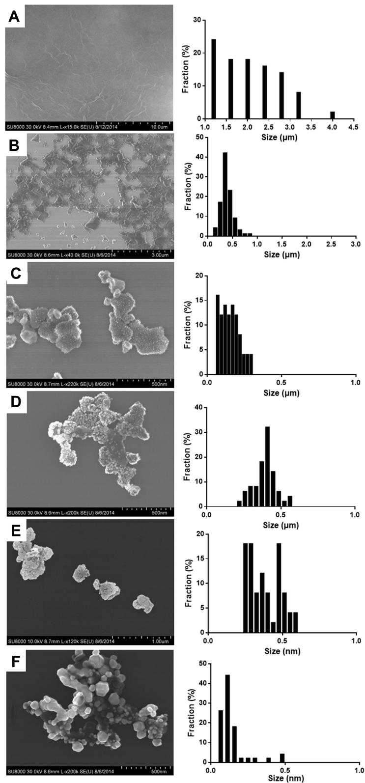
Figure 1 SEM images and size distribution of GO (A), GO@SiO 2 (B), GO@SiO 2 @Au seeds (C) and GO@SiO 2 @AuNS with different amount of 1 mL (D), 2 mL (E) and 4 mL (F) of HAuCl 4 . The right panels are the size distributions of these nanomaterials by measuring at least 100 nanomaterials.
