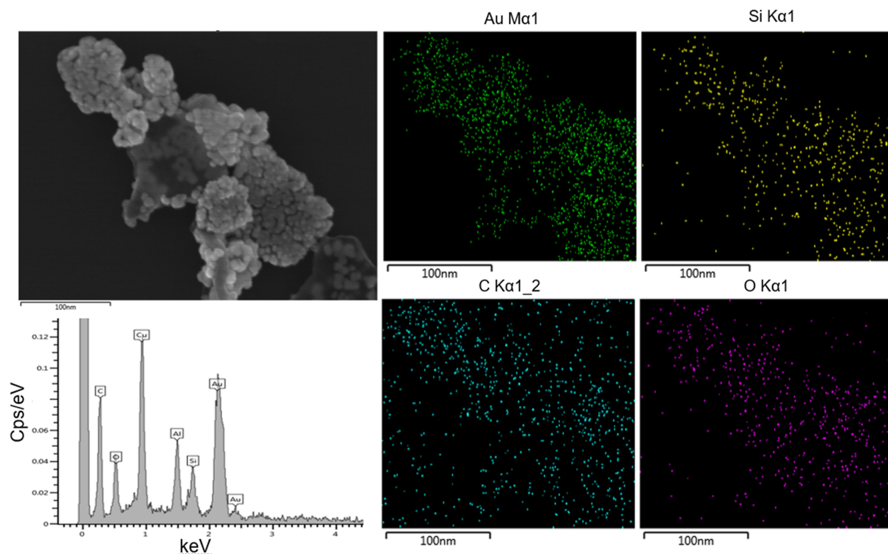
Figure 3 EDS map pattern and spectrum of the GO@SiO 2 @AuNS hybrid.
