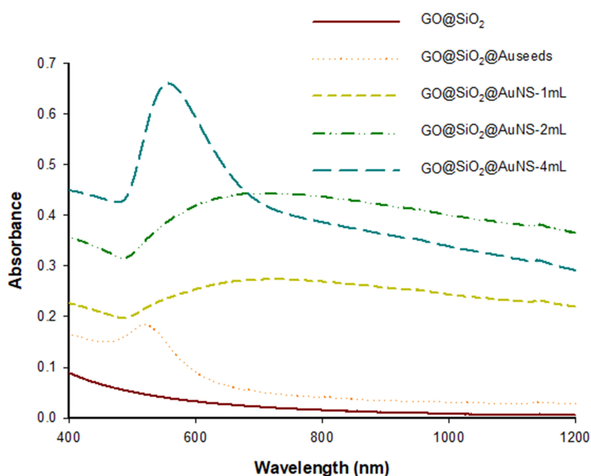
Figure 4 The absorption spectra of the synthesized nanomaterials.
