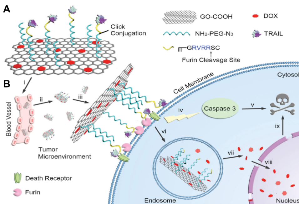
Figure 2 Scheme of TRAIL/DOX-fGO nanoplateform. (A) Main components of TRAIL/DOX-fGO, and (B) Step by step activity of TRAIL/DOX-fGO, from vessel administration to drug release in the cell nucleus.
