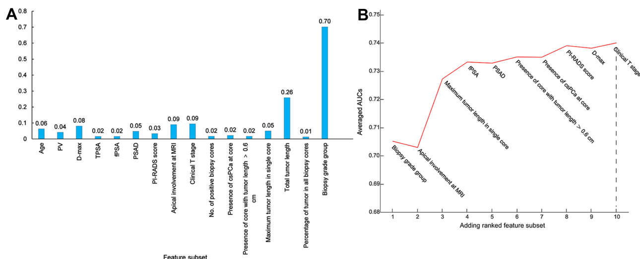
Figure 2 Results of feature selection, feature ranking, and model construction with RFE-SVM analysis. ( A ) Distribution of weight for features with RFE-SVM analysis. ( B ) Influence on AUC with incrementally adding ranked features in RFE-SVM. RFE-SVM classifier is trained by adding ranked feature one by one. The iteration repeated until the desired number of features was reached.
