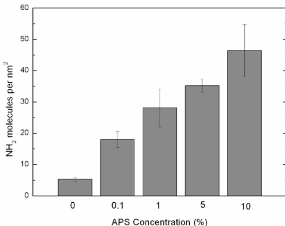
Figure 4 The application of the ninhydrin test to quantify the concentration of amine groups available on the surface of a silica microsphere.
