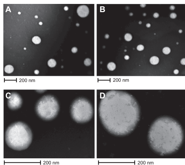
Figure 1 Photographs of TEM. A) and C) ZnPc-loaded PCL nanoparticles; B) and D) empty nanoparticles.
