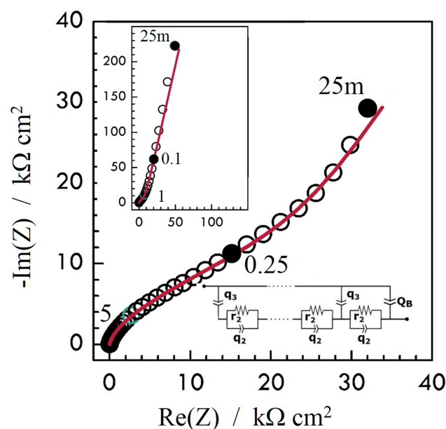
Figure 5 Nyquist plot of experimental (symbols) and fitted (solid lines) impedance spectroscopy of annealed layers LL cr (main plot) and SS cr (upper inset) measured in SBF electrolyte at open circuit conditions, 36.5 °C, in the dark. Frequencies in Hz. Bottom inset: Electrical equivalent circuit based used for fitting the experimental diagrams. q_2 and r_2 represent the nanotube solid channel's internal distributed resistance and non-ideal capacitance, q_3 the nanotube's wall interfacial capacitance, and Q_b the non-ideal dense layer capacitance.
