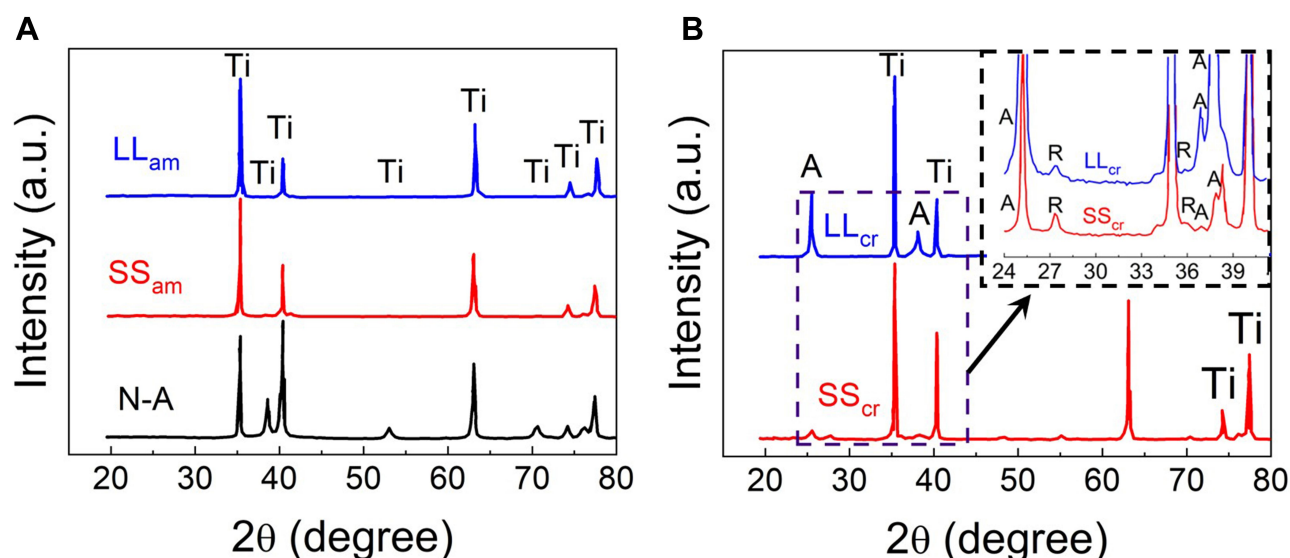
Figure 1 XRD patterns of different samples: (A) not-anodized, N-A, and as-anodized SS_{am} and LL_{am} and (B) annealed in air at 550 °C for 2 h ( SS_{cr} and LL_{cr} ). In the inset: zoom at 24^{\circ} < 2\theta < 42^{\circ} indicating the crystallization of both morphologies into a mix of anatase (A) and rutile (R).
