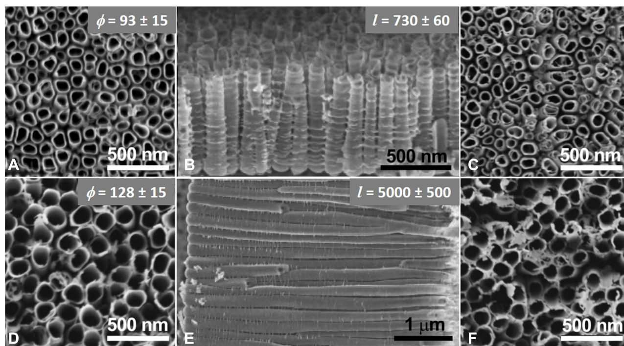
Figure 2 SEM images of the different TiO_2 nanotubes morphologies according to anodizing protocols SS (A–C) and LL (D–F). As-anodized samples: SS_{am} top (A) and cross-section (B) views and LL_{am} top (D) and cross-section (E) views. Annealed in the air at 550 °C for 2 h: SS_{cr} (C); LL_{cr} (F). Dimensions in nm expressed as \bar{x} \pm \sigma_x .
