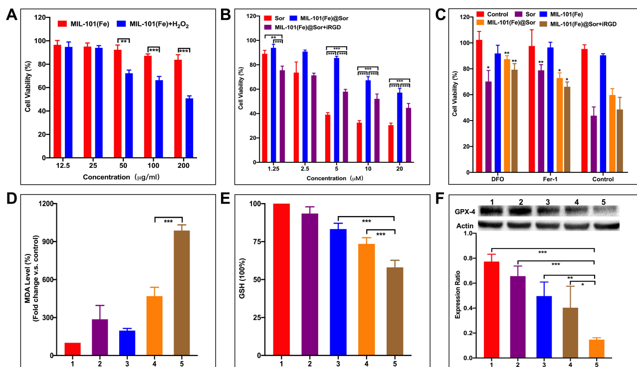
Figure 4 Mechanism of MIL-101(Fe)@sor-induced ferroptotic cell death. (A) and (B) MTT viability assays of HepG2 cells with different treatments. (C) MTT viability assays of HepG2 cells with different treatments and ferroptosis inhibitors. (D) and (E) MDA and GSH levels in HepG2 cells after different treatments. (F) WB analysis of GPX4 expression in HepG2 cells after different treatments. 1–5: control, MIL-101(Fe), sorafenib, MIL-101(Fe)@sor, and MIL-101(Fe)@sor + iRGD groups, respectively. * p < 0.05, ** p < 0.01, *** p < 0.001.
