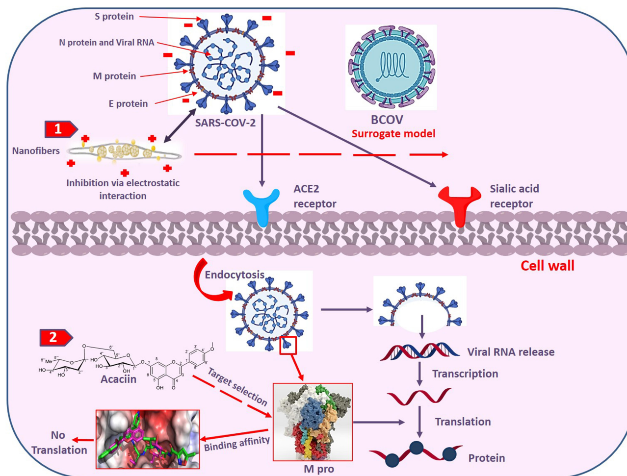
Figure 10 Cartoon summary for the two predicted pathways for inhibition of SARS-COV-2, 1) electrostatic binding of the NFs with the microbial envelop, 2) release of acaciin from the NFs and binding to the M pro which inhibits translation of polyproteins from the viral RNA and stops viral replication.
