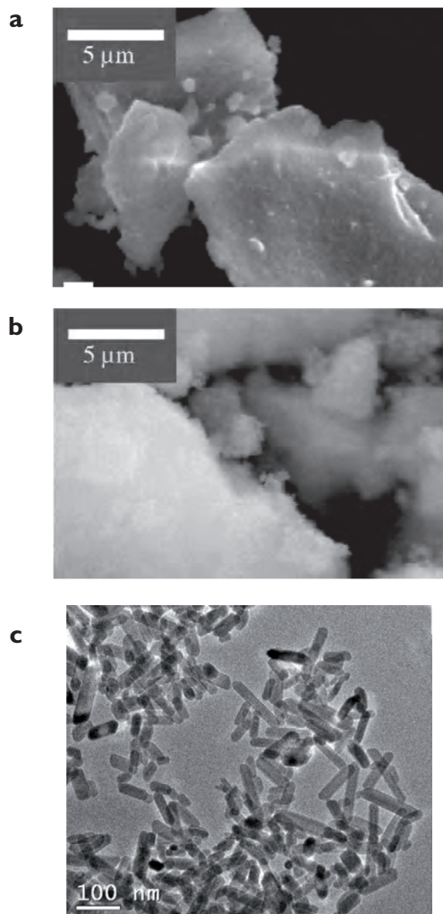
Figure 2 SEM images of (a) conventional (or micron grain size) and (b) nanometer grain size HA as well as a (c) TEM image of nanometer grain size HA. These HA particles were used in composite formulations. Abbreviations: HA, hydroxyapatite.
