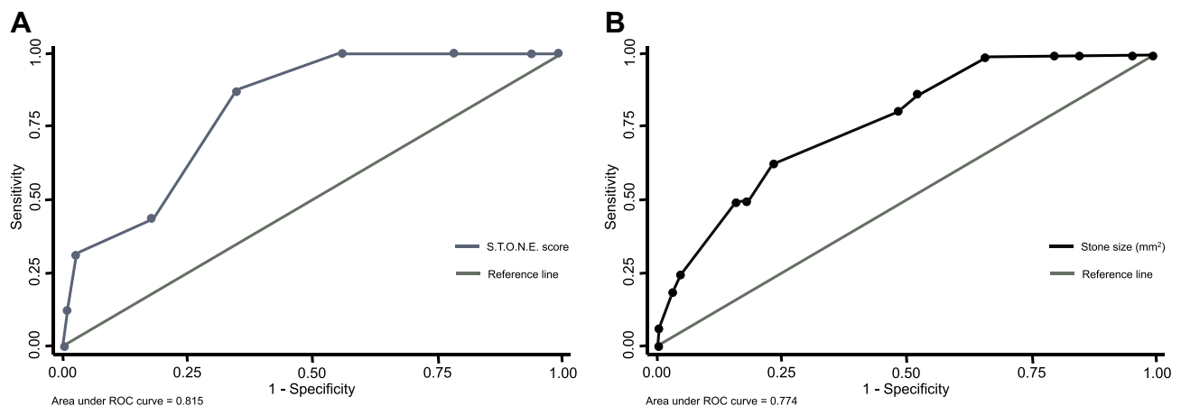
Figure 2 External validation of S.T.O.N.E. scoring system. (A) ROC curve of S.T.O.N.E. score. (B) ROC curve of stone size.
