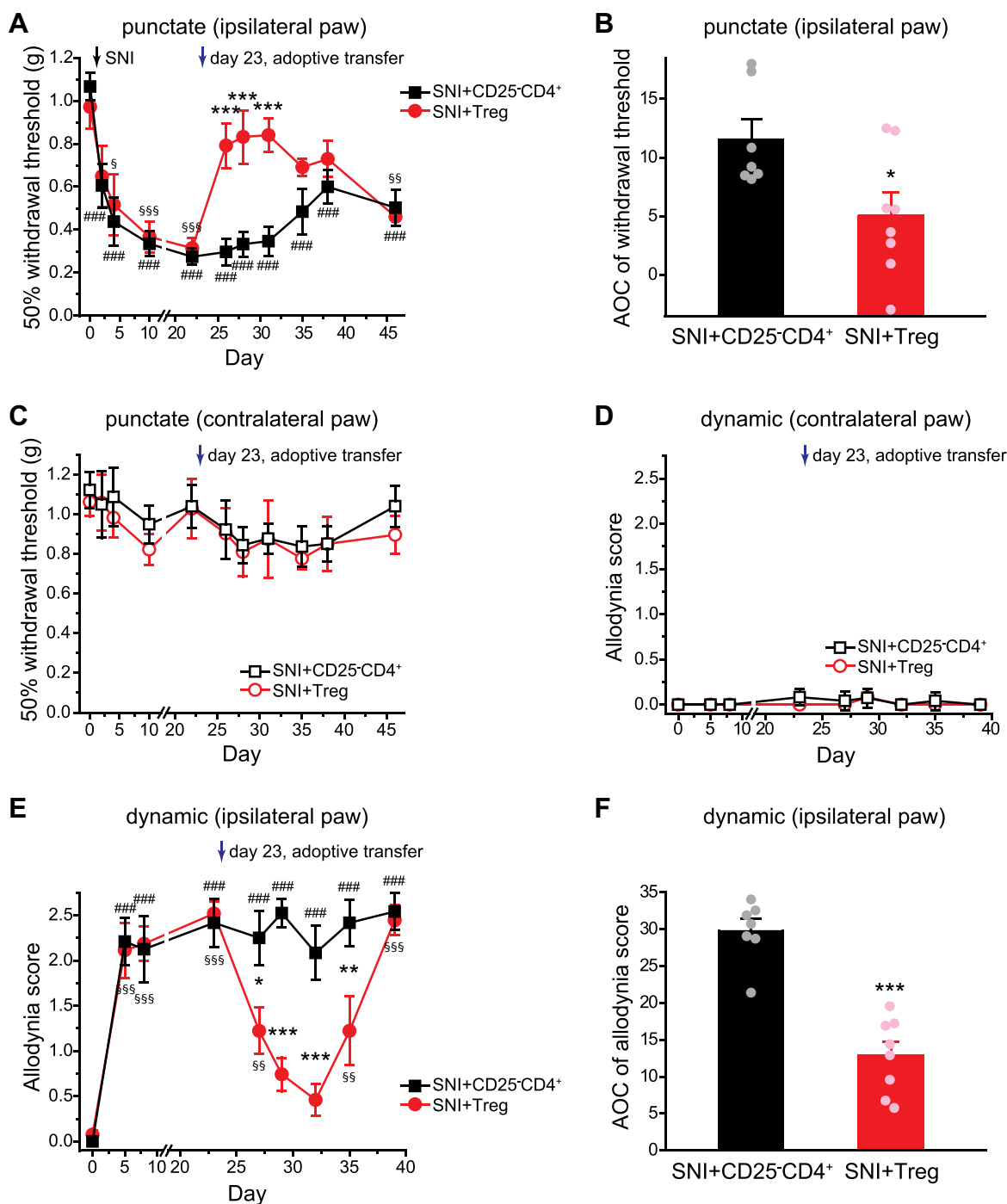
Figure 3 Adoptive transfer of Treg cells reverses the morphine-resistant punctate and dynamic mechanical allodynia. (A) Changes of the 50% withdrawal thresholds to von Frey filaments on the ipsilateral (right) hindpaws of male C57BL/6J mice ( n = 7-8 mice/group). SNI was performed on the right sciatic nerve on day 0, after the baseline measurement. On day 23, mice received adoptive transfer of Treg cells or CD25 + CD4 + cells as indicated by the arrow. Two-way RM ANOVA: p < 0.05 between groups; post hoc Student-Newman-Keuls test: ***p < 0.001 , between the corresponding SNI+CD25 + CD4 + and SNI+Treg groups; One-way RM ANOVA: p < 0.001 within the SNI+CD25 + CD4 + and SNI+Treg groups; post hoc Dunnett's test: ####p < 0.001 , compared with the baseline threshold (day 0) in the SNI+CD25 + CD4 + group; §p < 0.05 , §§p < 0.01 , §§§p < 0.001 , compared with the baseline threshold (day 0) in the SNI+Treg group. (B) The integrated AOCs of withdrawal threshold calculated from day 26 to day 45 post-SNI (same mice as in A ). *p < 0.05 , two-tailed t-test. (C) The 50% withdrawal thresholds to von Frey filaments on the contralateral (left) hindpaws (same mice as in A ). Two-way RM ANOVA: p = 0.32 between groups. (D) The responses to brush stimuli on the contralateral (left) hindpaws (same mice as in A ). Two-way RM ANOVA: p = 1.00 between groups. (E) SNI- and Treg transfer-induced changes of the dynamic allodynia scores of the ipsilateral (right) hindpaws of male C57BL/6J mice (same mice as in A ). Two-way RM ANOVA: p < 0.001 between groups; post hoc Student-Newman-Keuls test: *p < 0.05 , **p < 0.01 , ***p < 0.001 , between the corresponding SNI+CD25 + CD4 + and SNI+Treg groups; One-way RM ANOVA: p < 0.001 within SNI+CD25 + CD4 + and SNI+Treg groups; post hoc Dunnett's test: ####p < 0.001 , compared with the baseline score on day 0 in the SNI+CD25 + CD4 + group; §p < 0.01 , §§p < 0.001 , compared with the baseline score in the SNI+Treg group. (F) The integrated AOCs of dynamic allodynia score calculated from day 27 to day 39 post-SNI (same mice as in A ). ***p < 0.001 , two-tailed t-test. Abbreviations: Treg, regulatory T cell; SNI, spared nerve injury; RM ANOVA, repeated measures analysis of variance; AOC, area over the time-effect curve.
