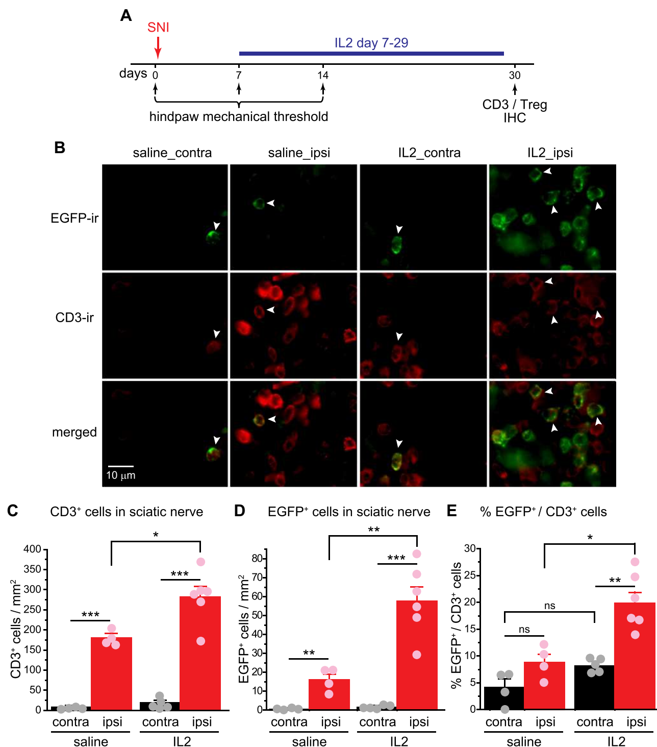
Figure 4 Ld-IL2 treatment preferentially increases the ratio of Treg cells to total CD3 + T cells in the injured sciatic nerve. (A) Time line of the experiment. Note that IL2 was always injected after the completion of behavioral tests on the same day. (B) Representative images of EGFP + and CD3 + and cells in the sciatic nerves ipsilateral (ipsi) and contralateral (contra) to the SNI surgery in female DREG mice at day 30 post-SNI. (C and D) The densities of CD3 + T cells (C) and EGFP + Treg cells (D) in the ipsilateral and contralateral sciatic nerves of female DREG mice at day 30 post-SNI. Mice were treated with daily Ld-IL2 or saline between day 7 and 29 post-SNI ( n = 6 and 4 , respectively). * p < 0.05 , ** p < 0.01 , *** p < 0.001 , two-way ANOVA and post hoc t -test with Bonferroni correction. (E) The fraction of EGFP + Treg cells among CD3 + T cells in the sciatic nerves ipsilateral and contralateral to the SNI surgery (same mice as in C and D ). * p < 0.05 , ** p < 0.01 , two-way ANOVA and post hoc t -test with Bonferroni correction.
