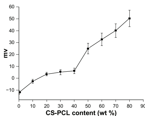
Figure 4 Zeta-potential curve for electrospun nanofibrous scaffolds ( n = 5 ). Abbreviation: CS-PCL, cationic chitosan-graft-poly ( \epsilon -caprolactone).
