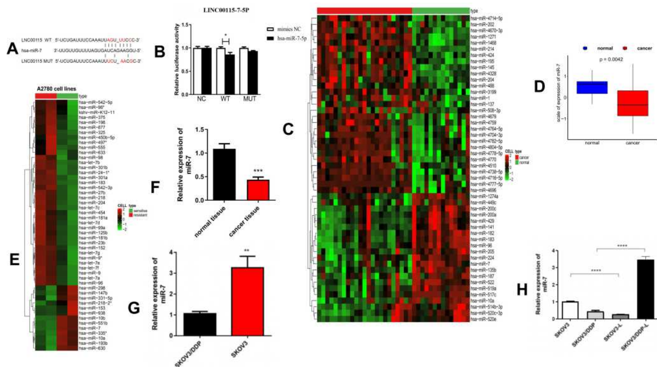
Figure 2 LNC00115 sponges miR-7 in ovarian cancer cells. (A and B) Dual-luciferase assays were performed to confirm the binding of LNC00115 to miR-7. (C) Hierarchical clustering heat map of differential miR-7 expression in ovarian tissues and corresponding normal tissues generated from the GEO database (GSE53829). (D) The expression of miR-7 in an ovarian cancer cohort and normal tissue cohort obtained from the GEO database (GSE53829). (E) Hierarchical clustering heat map of differential miR-7 expression in A2780-DDP and A2780 ovarian cells from the GEO database (GSE84201). (F) qRT-PCR analysis of miR-7 expression in ovarian cancer tissues and normal tissues, P = 0.0007 . (G) qRT-PCR analysis of miR-7 expression in SKOV3-DDP and SKOV3 cells, P = 0.0025 . (H) qRT-PCR analysis of miR-7 expression in SKOV3, SKOV3-DDP, SKOV3-L, and SKOV3-DDP-L cells. Data represent the means \pm SD. * P < 0.05 , ** P < 0.01 , *** P < 0.001 and **** P < 0.0001 .
