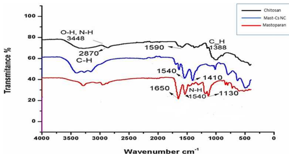
Figure 4 Fourier transform infrared spectra of Mast-Cs NC, chitosan and mastoparan. The y-axis shows the percent transmittance and the x-axis the wave number (cm -1 ). The spectrum of raw chitosan (black line) indicates the characteristic broad absorption peak at 3448 cm -1 , which corresponds to the amino and hydroxyl group stretching vibrations (N–H and O–H bonds, stretch). The peak at 2870 cm -1 is responsible for –CH 2 stretching (C–H bond, stretch). The characteristic bend at 1388 cm -1 shows the C–H bend. Mastoparan (red line) shows angular deformations at the N–H bonds of the amino groups at 1540 cm -1 . The spectrum of Mast-Cs NC (blue line) indicates conformational change in peaks/bands; the N–H and O–H peak has broadened at 3200 cm -1 , and N–H bands/peaks have widened at 1540–1590 cm -1 ; the 1130 cm -1 peaks have disappeared, owing to the interaction between mastoparan and the polymeric structure of chitosan.
