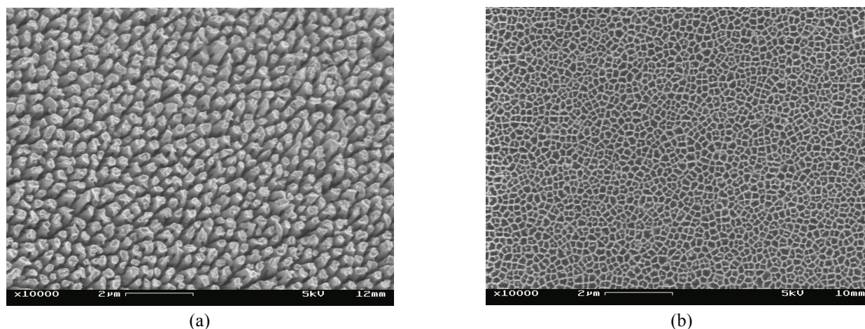
Figure 1 SEM images show top-view of the nanostructured substrates with nanopillars (a) and nanopores (b). Abbreviations: SEM, scanning electron microscope.
