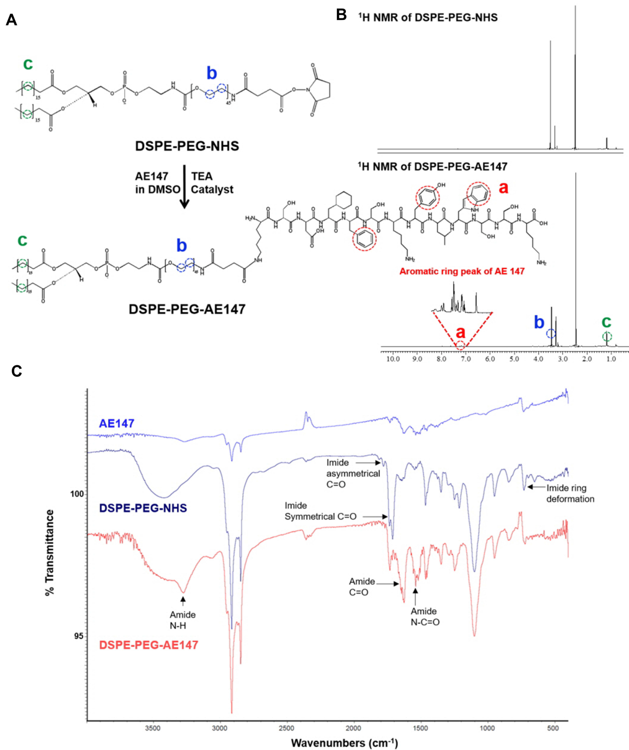
Figure 2 (A) Synthesis scheme of DSPE-PEG-AE147. (B) ^1\text{H NMR} spectra of DSPE-PEG-NHS and DSPE-PEG-AE147. (C) FT-IR spectra of AE147, DPSE-PEG-NHS, and DSPE-PEG-AE147.
