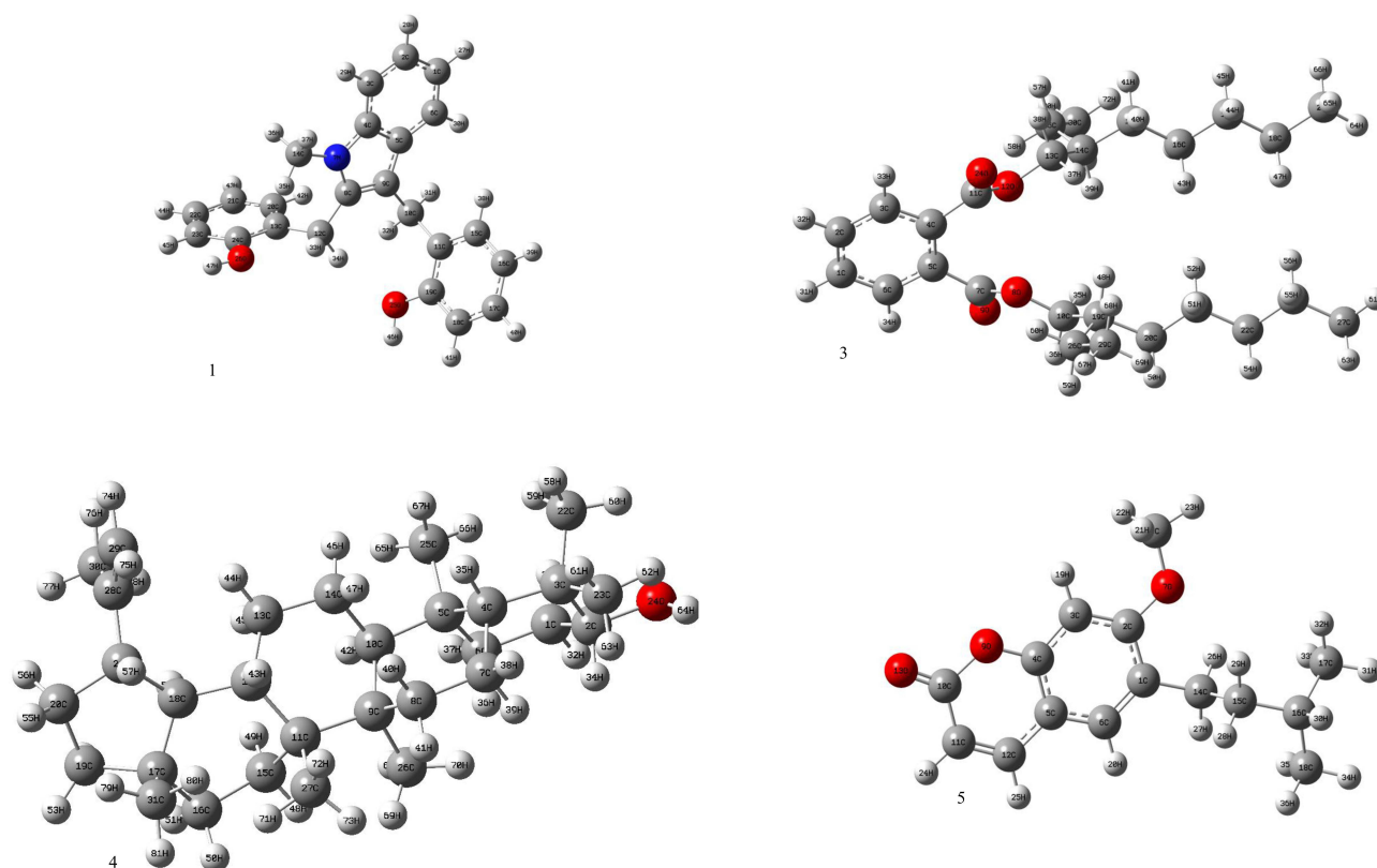
Figure 5 The optimized structures of compounds 1 , 3–5 .
