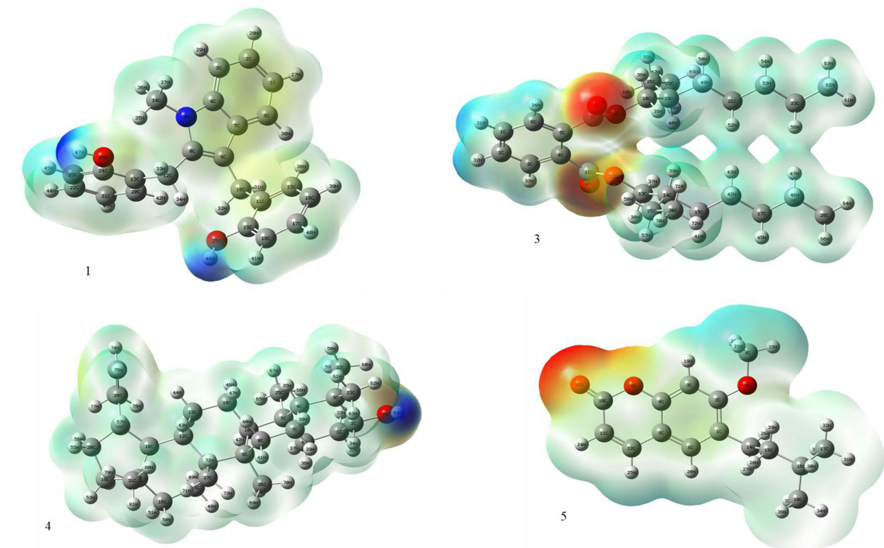
Figure 6 Molecular electrostatic potential surface of compounds 1 , 3–5 .
