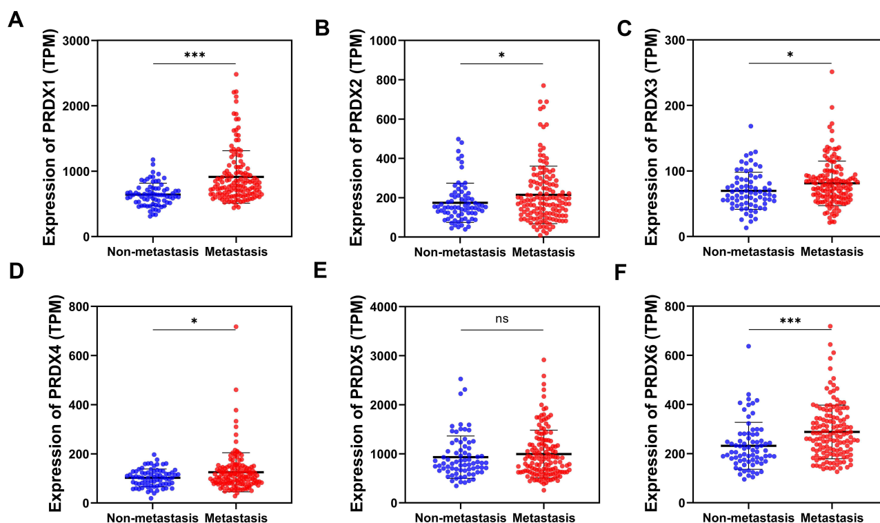
Figure 2 The expression levels of PRDX family of non-metastasis group (blue) and metastasis group (red) in OSCC (TCGA cohort). (A) PRDX1; (B) PRDX2; (C) PRDX3; (D) PRDX4; (E) PRDX5; (F) PRDX6. * P < 0.05 ; *** P < 0.001 .
