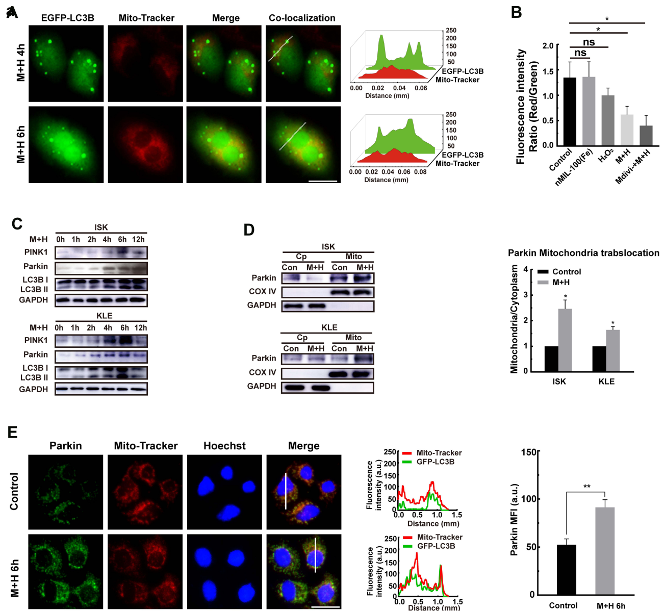
Figure 5 PINK1/Parkin mediated-mitophagy activation by nMIL-100 (Fe) and H 2 O 2 nanosystem. (A) The fluorescence images of GFP-LC3B-transfected ISK cells after treatment with 100 \mu M nMIL-100 (Fe) and 50 \mu M H 2 O 2 for 4 h or 6 h followed by Mito-Tracker (red) incubation (scale bar is 20 \mu m). The colocalization between green spots and red mitochondria tracker was elevated by Plot Profile tool. (B) Quantifications of the mitochondrial membrane potential (MMP) \Delta\Psi_m (JC-1 red/green fluorescence intensity ratio) after different treatment including control, 100 \mu M nMIL-100 (Fe) alone, 50 \times 10^{-6} M H 2 O 2 alone, a combination of both or a pretreatment of Mdivi-1 (5 \times 10^{-6} M, 1 h) before the both additions for 24 h. (C) Western blot analysis of PINK1, Parkin, LC3-I and LC3-II expression in ISK and KLE cells treated with 100 \mu M nMIL-100 (Fe) and 50 \times 10^{-6} M H 2 O 2 for different time intervals, using GAPDH as loading control. (D) Parkin expression in mitochondrial and cytosolic enriched fractions of ISK and KLE cells after 100 \mu M nMIL-100 (Fe) and 50 \times 10^{-6} M H 2 O 2 treatment for 6 h was determined by Western blot, using GAPDH and COX IV as cytosolic and mitochondrial loading control respectively. (E) The images of immunofluorescence in ISK cells undergoing the same treatments as the aforementioned in (D) followed by co-staining with Mito-Tracker (red) and Hoechst 3342 (blue) (scale bar is 20 \mu m). The MFI of Parkin and the colocalization (white straight lines) between green Parkin and red mitochondria tracker was analyzed by Plot Profile tool. Data were represented as mean \pm SD (n=3). * p < 0.05, ** p < 0.01, ns, not significant.
