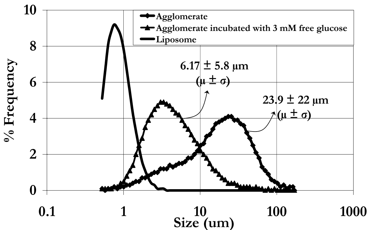
Figure 2 Size distributions measured by Fraunhofer Diffraction of con A-linked liposomes before and upon cleavage by free glucose.
