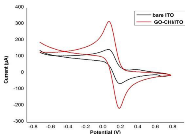
Figure 5 Cyclic voltammogram (CV) of bare ITO and GO-CHI/ITO electrodes at 100mV 1/2 .
