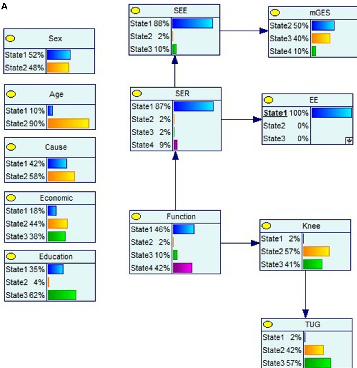
Figure 3 (A) Continued.
