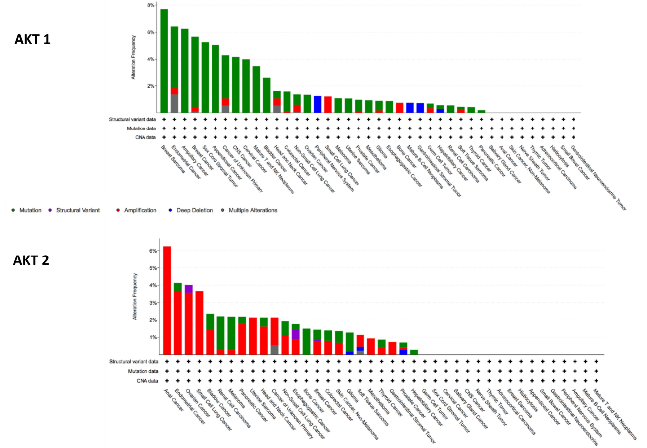
Figure 2 Frequency of AKT1 and AKT2 alterations from analysis of MSK-IMPACT Clinical Sequencing Cohort (MSKCC, Nat Med 2017), cBioPortal genomic database. 33,34
