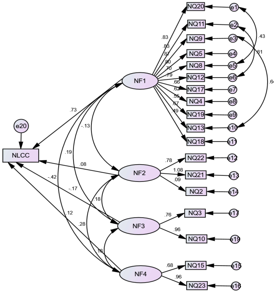
Figure 2 Effect of factor variables on NLCC.
