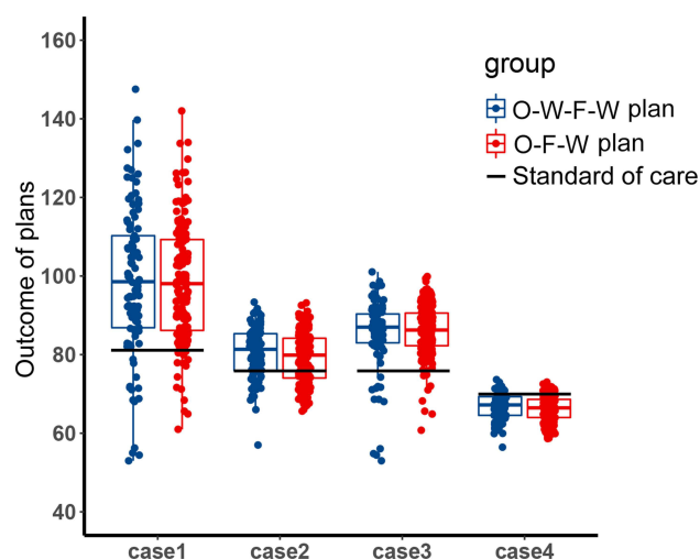
Figure 4 The distribution of the outcome of the filtered fixed periodic plans. Boxplot of the outcome of the O-W-F-W plans and O-F-W plans in four competitive cases. The black horizontal line was the outcome of the standard of care in the corresponding competitive case.
