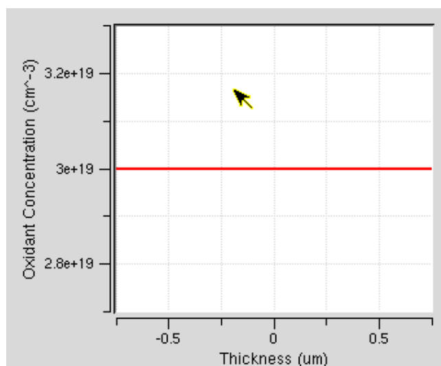
Figure 1 Oxidation flux of basophil. The transmembrane oxidant concentration is steadily equal to 3e + 19/\text{cm}^3 at any transmembrane ion concentration difference (thickness).
