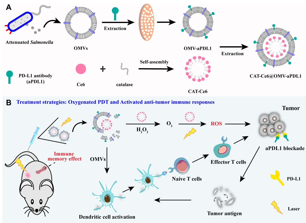
Scheme 1 Construction of CAT-Ce6@OMV-aPDL1 ( A ) and illustrations of promoted oxygenated PDT as well as activated anti-tumor immune responses induced by CAT-Ce6@OMV-aPDL1-based PDT and immunomodulation ( B ).
