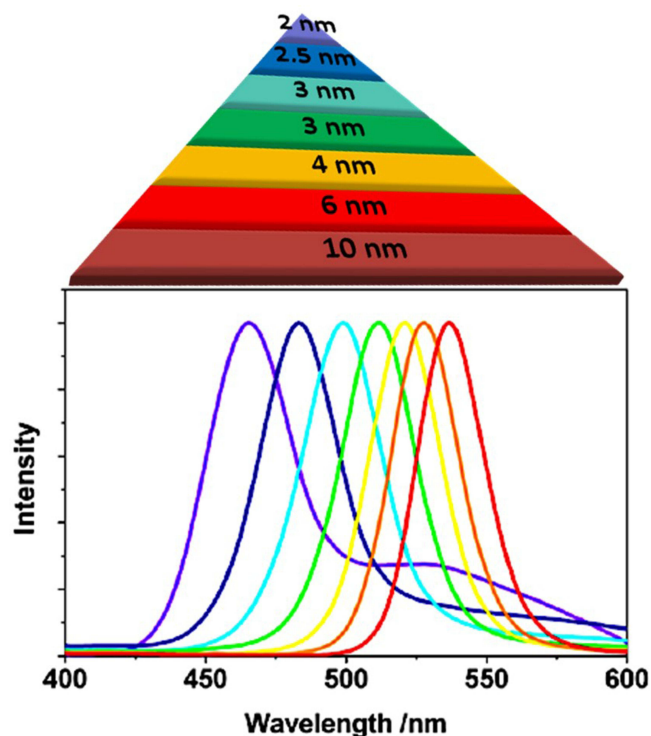
Figure 2 Impact of the particle size of CdSe QDs on their emission spectra upon irradiation with UV light. The emission wavelength is directly proportional to the particle size. Adapted from Bera D, Qian L, Tseng TK, Holloway PH. Quantum Dots and Their Multimodal Applications: A Review . 2010;3(4):2260–2345. Copyright © 2010 by the authors; licensee Molecular Diversity Preservation International, Basel, Switzerland. This article is an open-access article distributed under the terms and conditions of the Creative Commons Attribution license ( http://creativecommons.org/licenses/by/3.0/ ). 43
