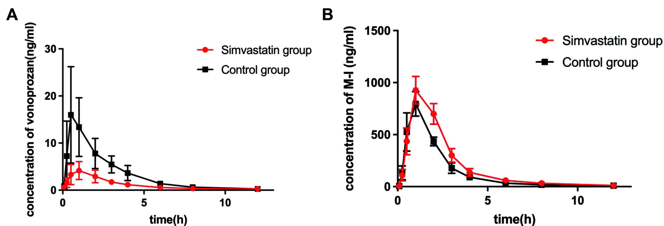
Figure 6 The concentration-time curves of vonoprazan (A) and M-I (B) in rat ( n = 6 ). The simvastatin group was injected with simvastatin intraperitoneally for 2 weeks and then administered with vonoprazan intragastrically; The control group was injected with saline only for 2 weeks and followed by administrated with same dose of vonoprazan to that of simvastatin pretreated group.
